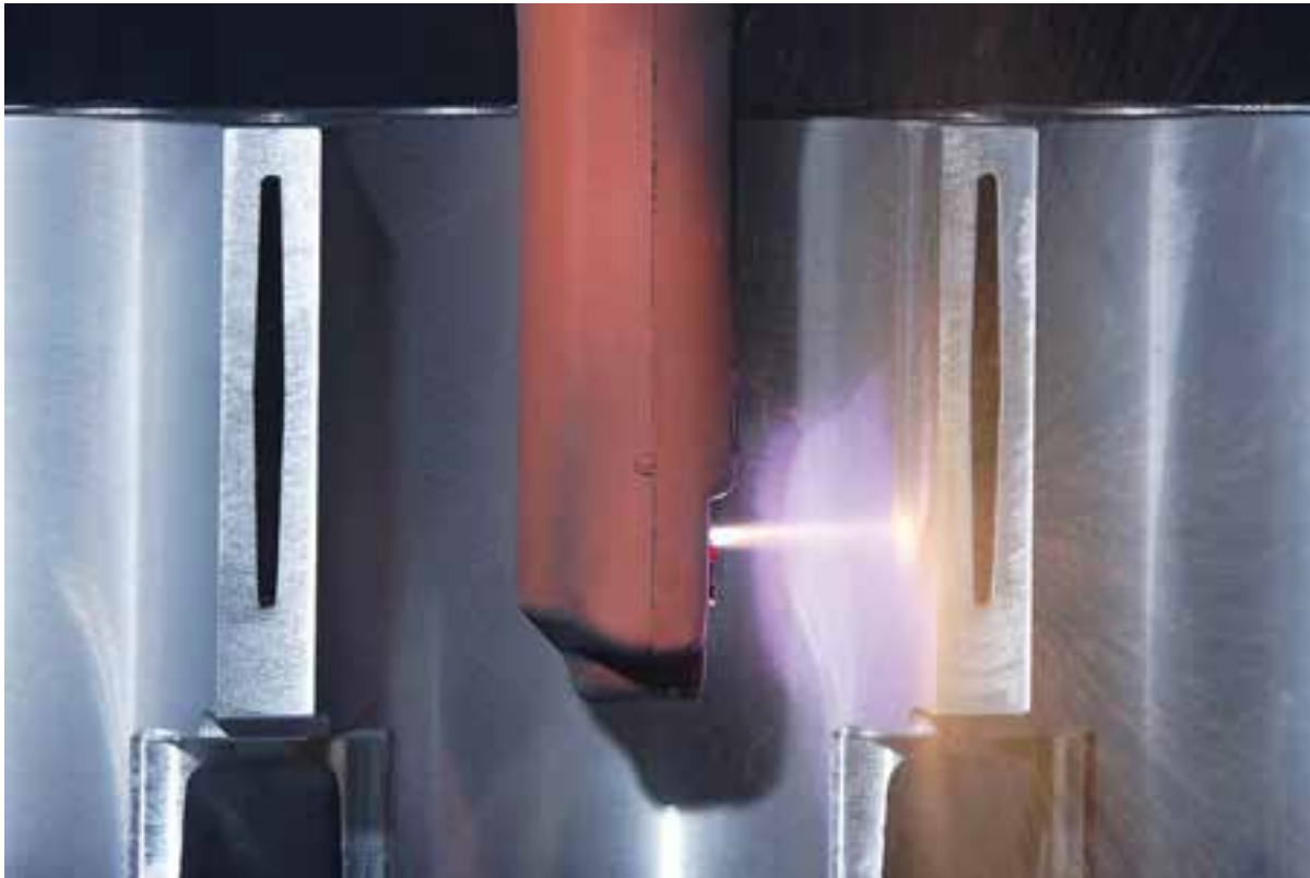
FIGURE 1. The cylindrical surface of a bore for an automobile engine is micromachined using a 2 kW single-mode fiber laser from IPG Photonics, then sprayed with plasma to create a hard coating that replaces conventional cylinder liners. Laser-machined microgrooves help the resulting coating to adhere to the cylinder. (Courtesy of IPG Photonics)
