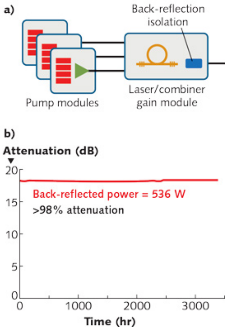
FIGURE 4. The nLIGHT alta design incorporates a back-reflection isolator between the laser and delivery fiber (a). A continuous laser-stability stress test with greater than 500 W directed back into the laser for thousands of hours shows no indication of unstable operation (b). (Courtesy of nLIGHT)
